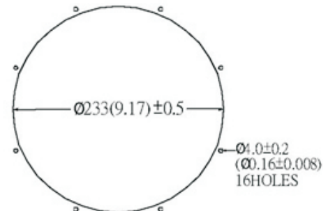
MOUNTION PANEL CUTOUT OUTLET SIDE & INLET SIDE
